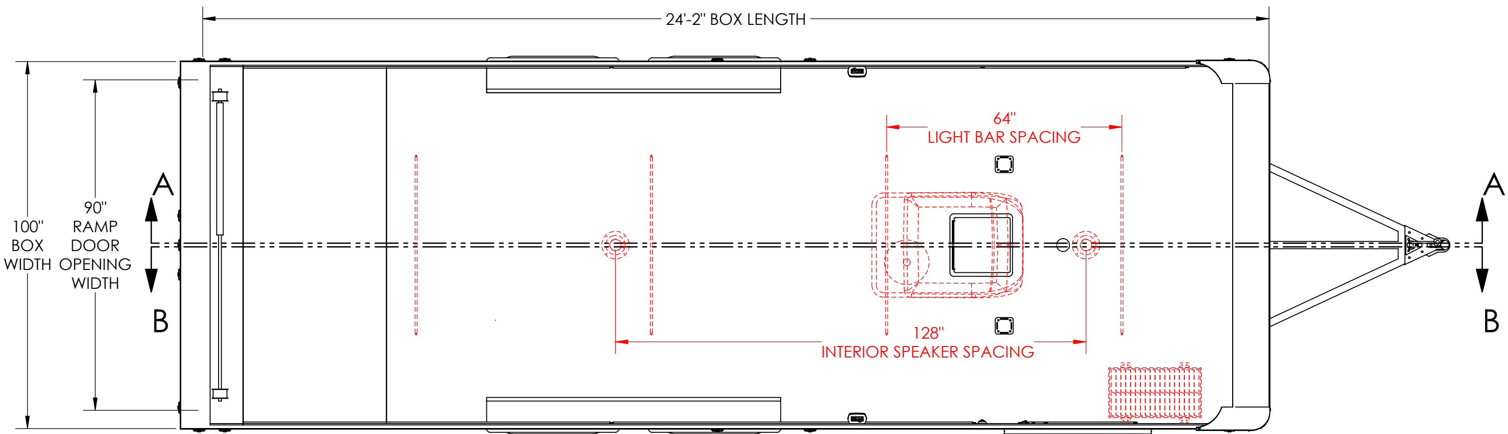
TOP VIEW ROOF & CEILING LAYOUT
